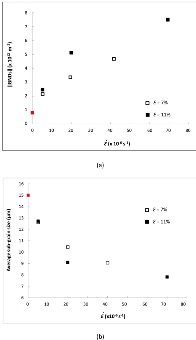
Fig. 9. (a) Average dislocation densities and (b) mean sub-grain size calculated from the EBSD maps of the two groups of pellets (D3, D6, D7) and (D5, D8, D9) respectively deformed to 7% and 11%. The red marker corresponds to the reference pellet R (with no sub-grains). (For interpretation of the references to color in this figure legend, the reader is referred to the Web version of this article.)
